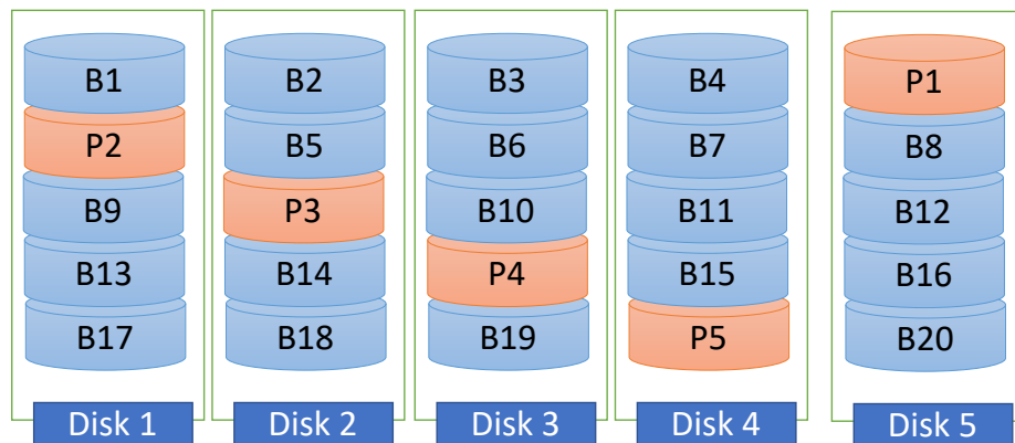
Figure 7.14: RAID 5
