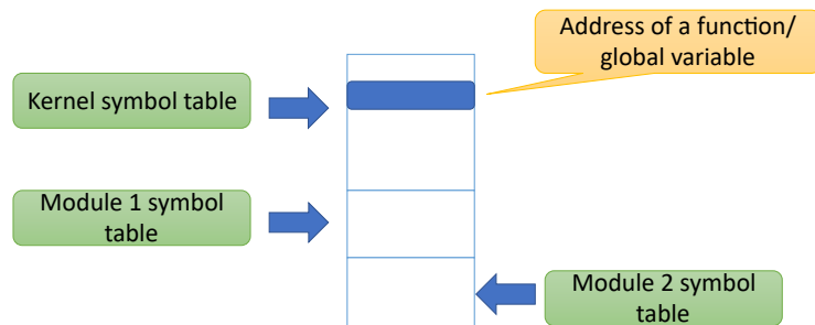
Figure 7.19: Kernel's global symbol table
