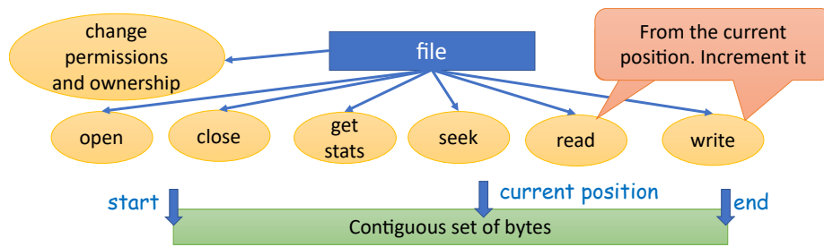
Figure 7.17: File operations in Linux
