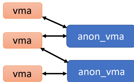
Figure 6.14: Many-to-many mapping
