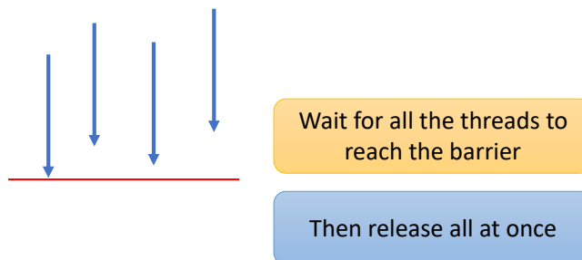
Figure 5.12: Barriers
