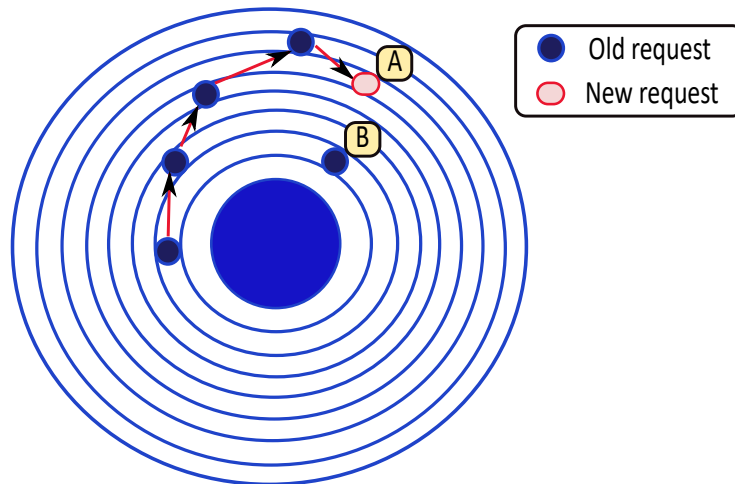
Figure 7.22: Example of the elevator algorithm, where fairness is being compromised. Fairness would require Request B to be scheduled before Request A because it arrived earlier. If we start servicing requests on the reverse path (outer to inner) then all the requests in the vicinity (nearby tracks) of A will get serviced first. Note that requests in the vicinity of A got two back-to-back chances: one when the head was moving towards the outermost track and one when it reversed its direction.
