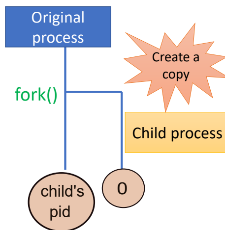
Figure 3.8: Forking a child process
