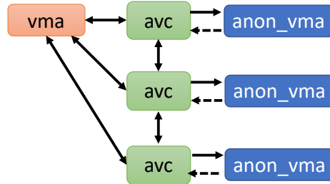
Figure 6.16: anon_vma_chain nodes connected together as a list (all corresponding to the same vma )
