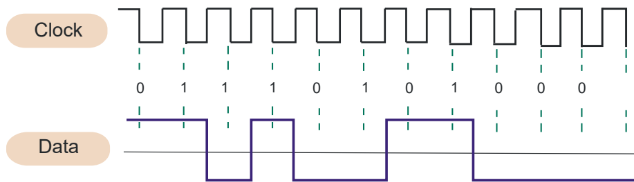
Figure 7.5: NRZI encoding
