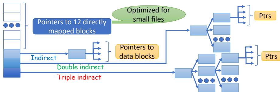
Figure 7.28: Structure of an ext4 inode
