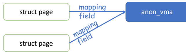
Figure 6.12: Pages pointing to an anon_vma
