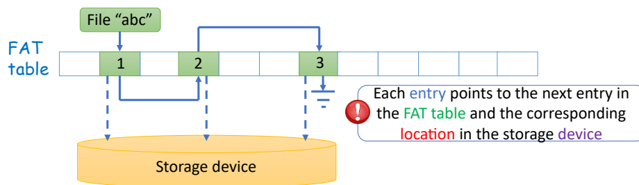
Figure 7.30: Mechanism of storing a file in the exFAT file system
