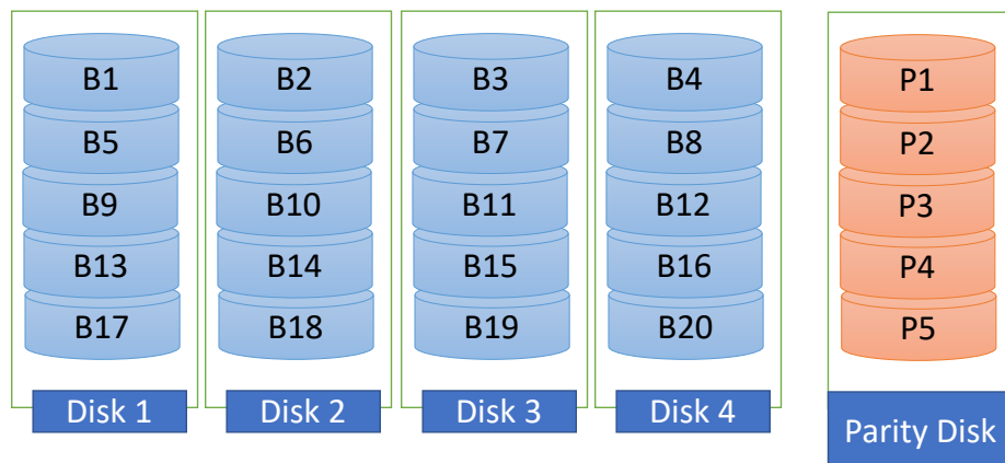
Figure 7.12: RAID 2, 3 and 4
