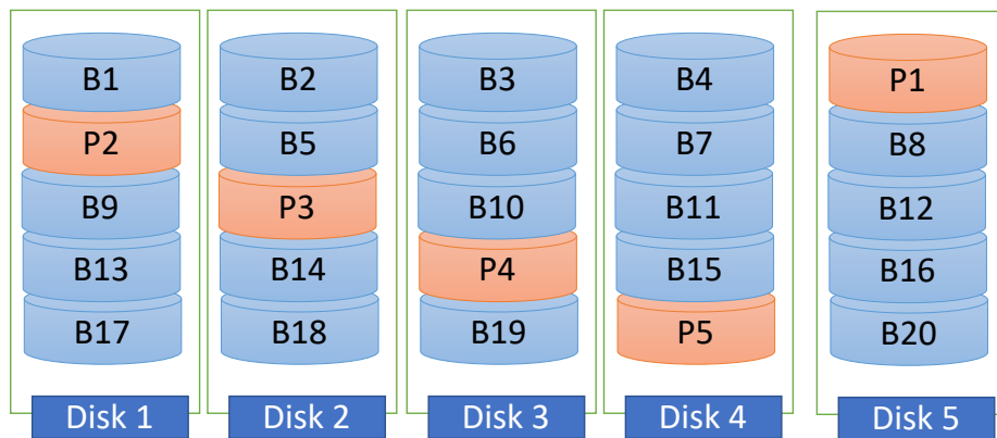
Figure 7.13: RAID 5
