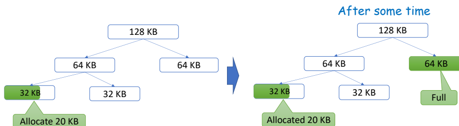
Figure 6.24: Buddy allocation
