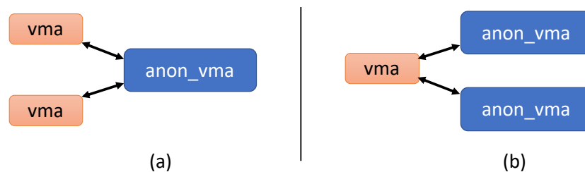
Figure 6.13: (a) Many-to-one mapping (b) One-to-many mapping
