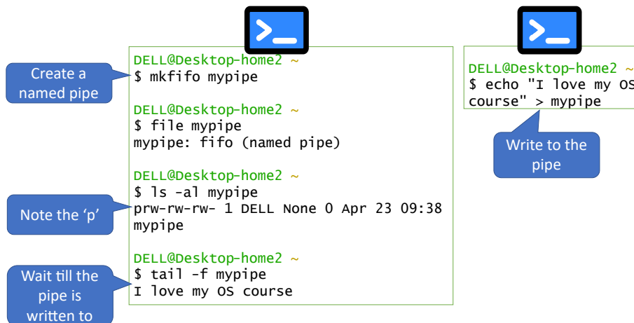
Figure 7.32: Pipes in Linux
