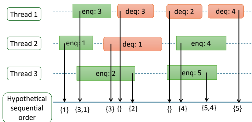
Figure 5.9: A parallel execution and its equivalent sequential execution. Every event has a distinct start time and end time. In this figure, we assume that we know the completion time. We arrange all the events in ascending order of their completion times in a hypothetical sequential order at the bottom. Each point in the sequential order shows the contents of the queue after the respective operation has completed. Note that the terminology enq: 3 means that we enqueue 3, and similarly deq: 4 means that we dequeue 4.
