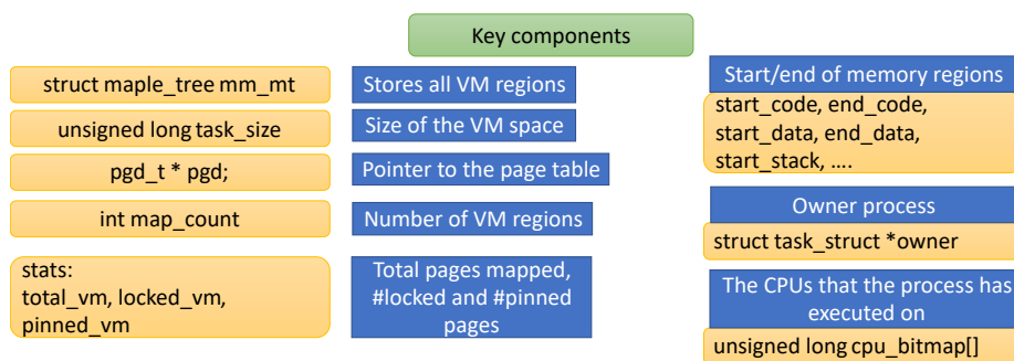
Figure 3.5: The key components of a process’s address space
