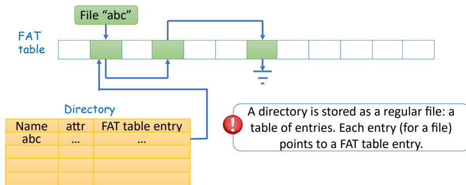
Figure 7.31: Storing files and directories in the FAT file system
