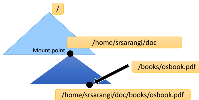
Figure 7.25: Mounting a file system
