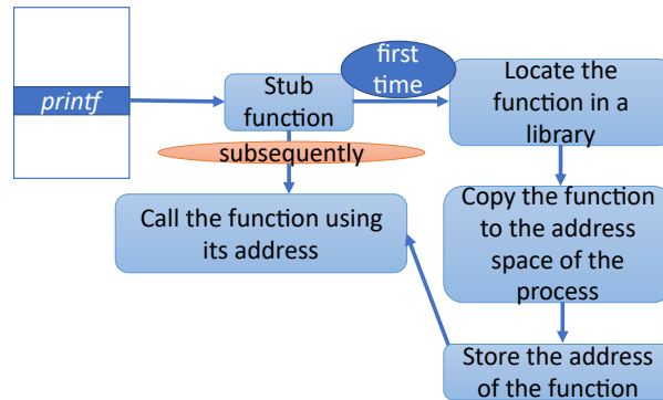
Figure B.5: Dynamically linking a program
