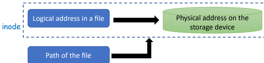
Figure 7.24: Notion of a mapping table (either pointed to by an inode or stored within it).
