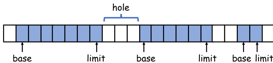
Figure 2.9: The base-limit scheme
