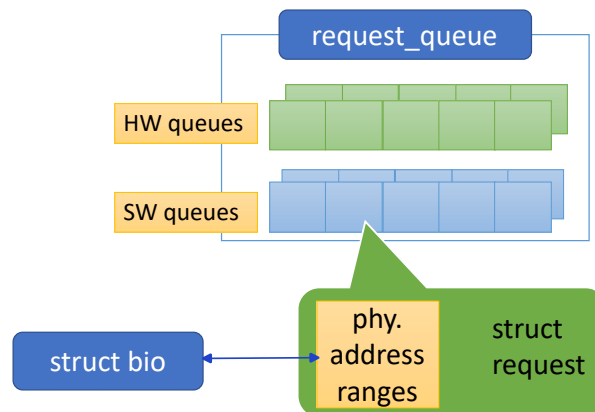
Figure 7.21: Request queues in the device driver subsystem
