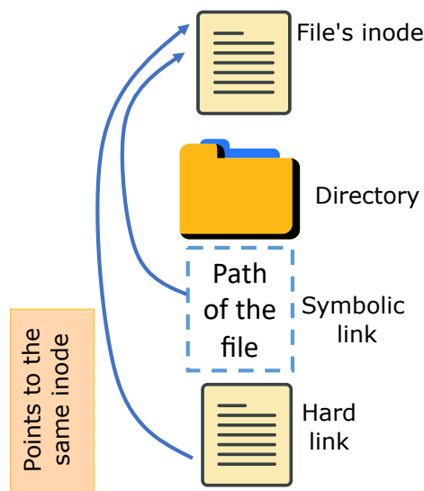
Figure 7.26: Hard and soft links
