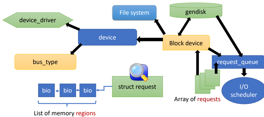
Figure 7.20: Kernel's block I/O system
