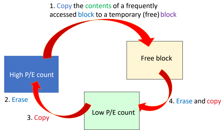
Figure 7.16: Block swap procedure
