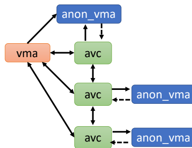
Figure 6.18: Example of a scenario with multiple processes where an anon_vma is associated with multiple vmas
