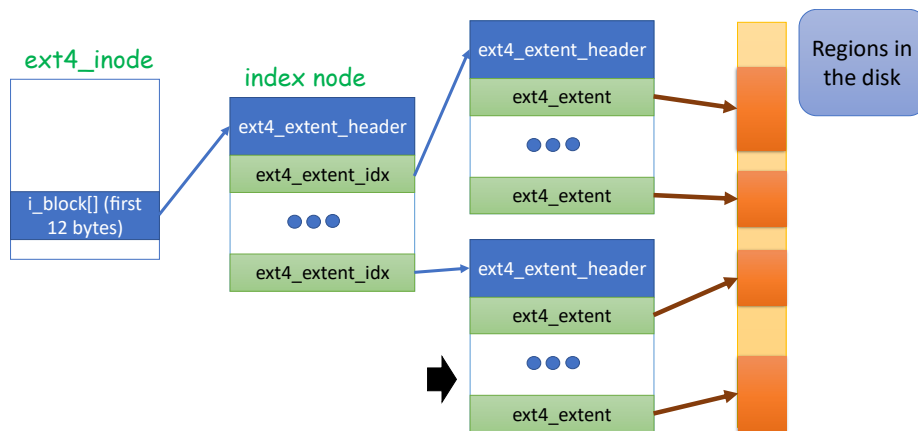
Figure 7.29: Structure of an ext4 inode with extents
