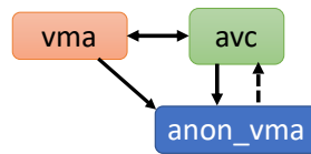
Figure 6.17: Updated relationship between vma , anon_vma and avc
