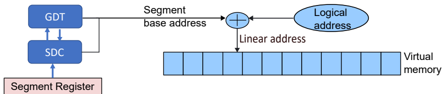
Figure 2.14: Computing the virtual address with memory segmentation
