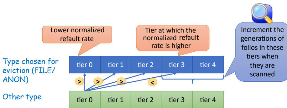
Figure 6.23: The notion of tiers
