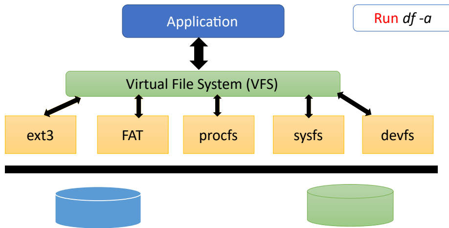
Figure 7.27: File systems supported by the Linux virtual file system (VFS).
